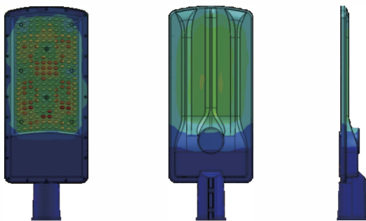
Thermal Conductivity
